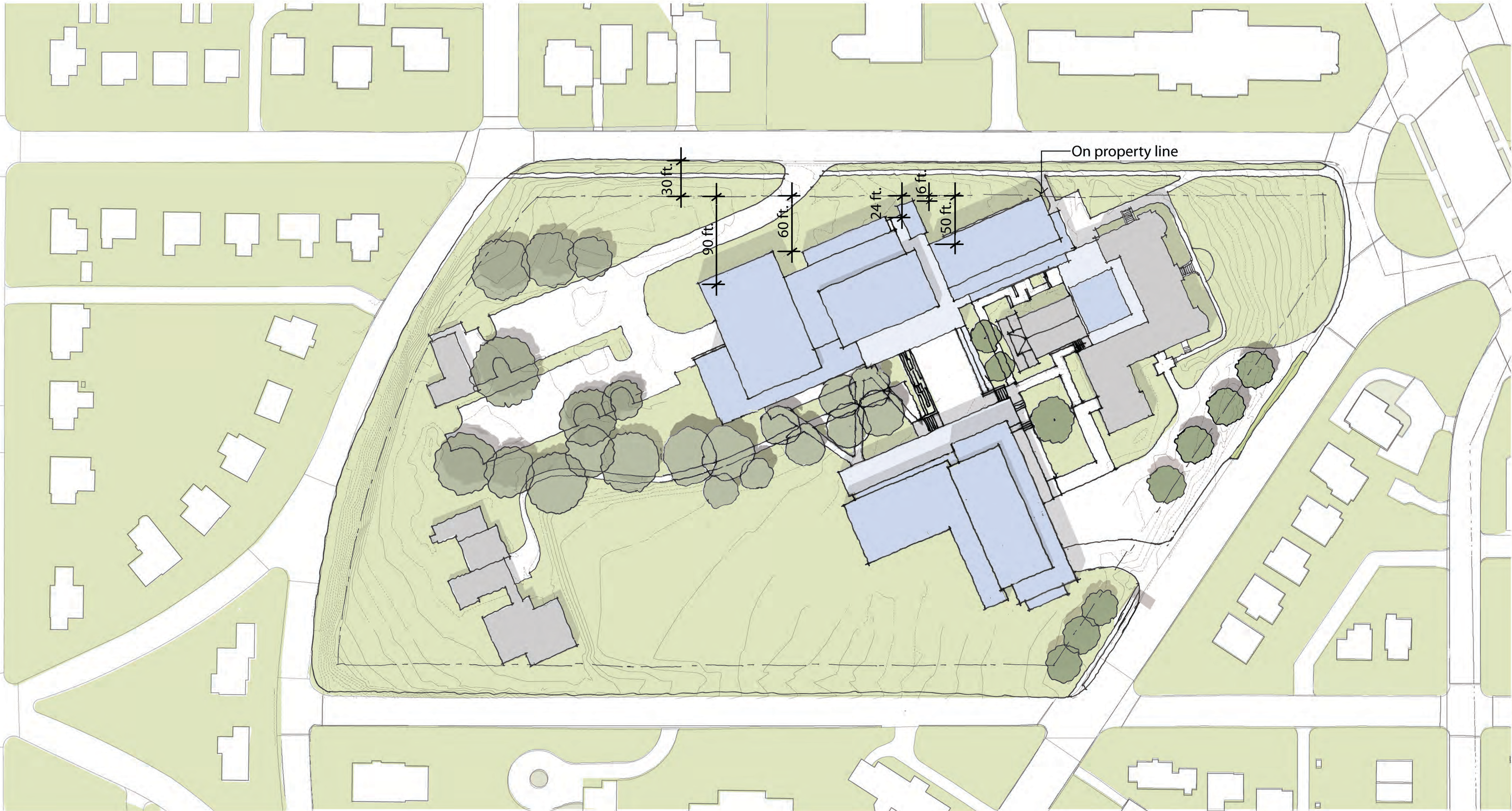
PROPOSED BUILDING SETBACKS ALONG YUMA
